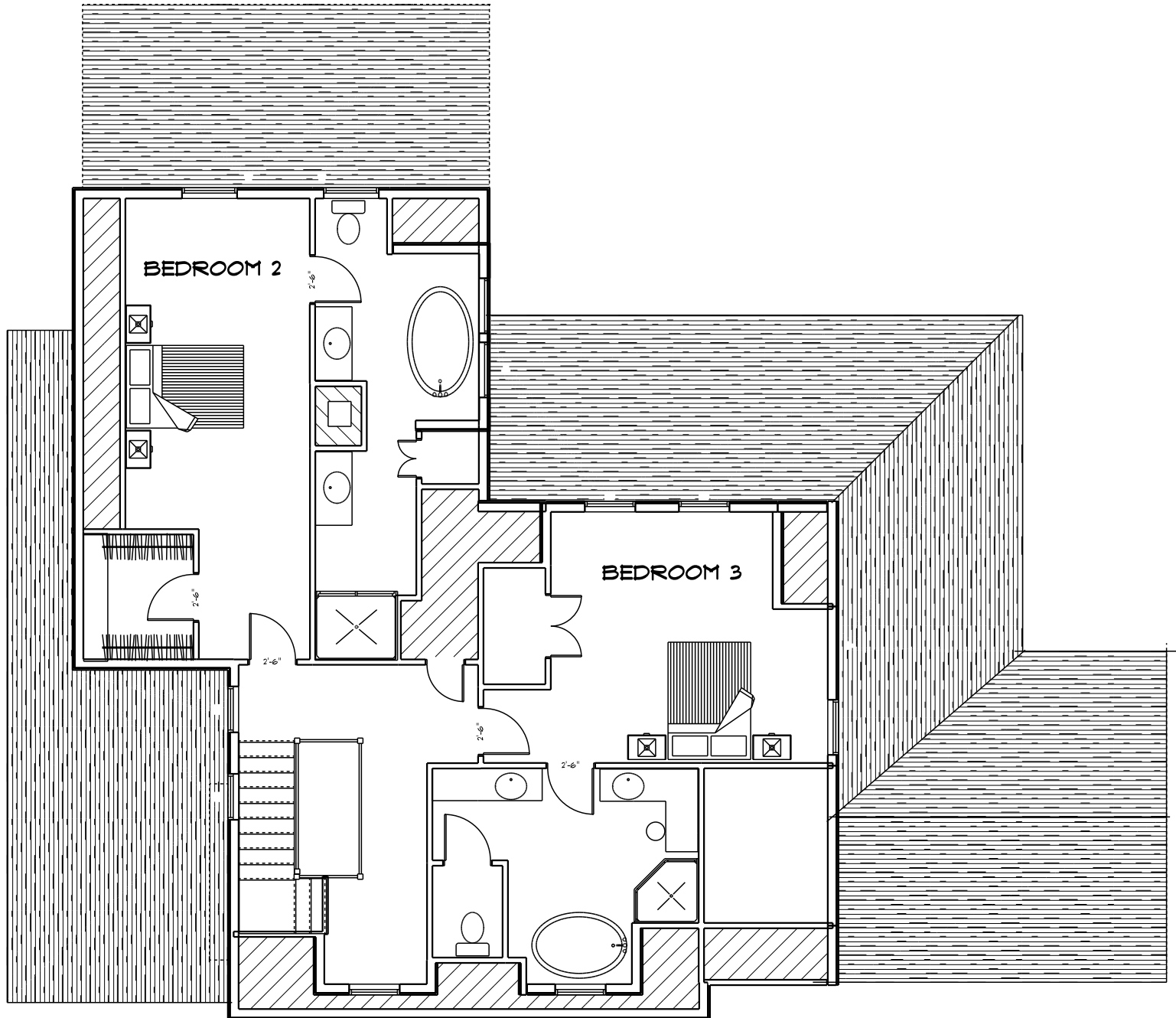
SECOND FLOOR 12-12-11
